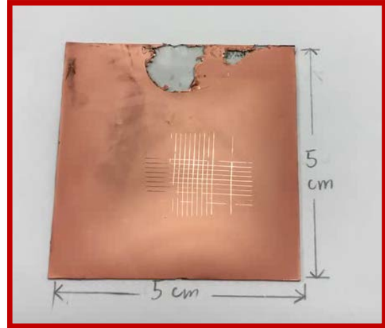
X Cut tape test following ASTM D3359, adhesion = 5B
