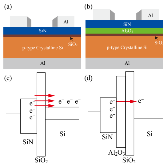
▲圖六 雙層(SiN/SiO 2 )及三層(SiN/ \text{Al}_2\text{O}_3 /SiO 2 )結構能帶示意圖
